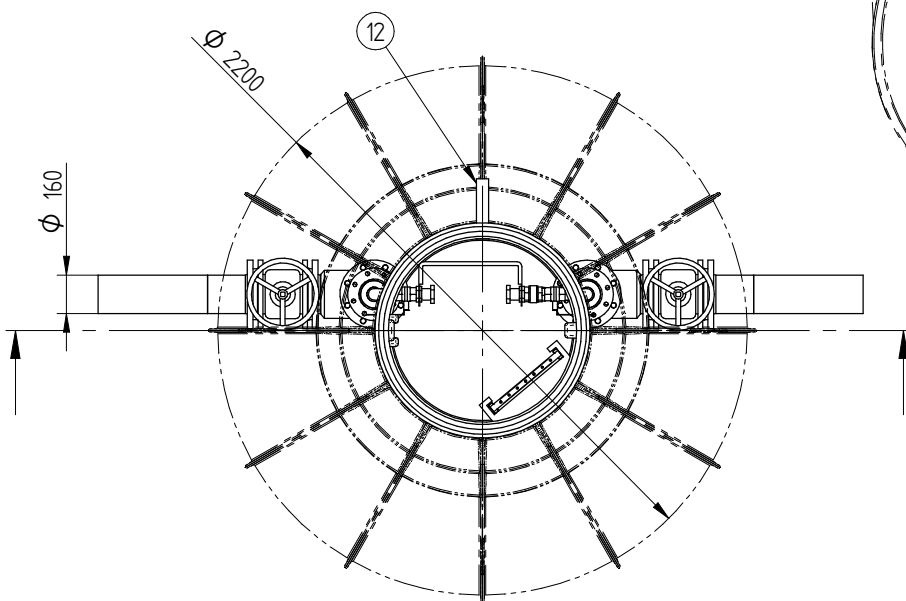
SECTION B-B
